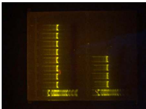
Figure 15: eDNA Results
