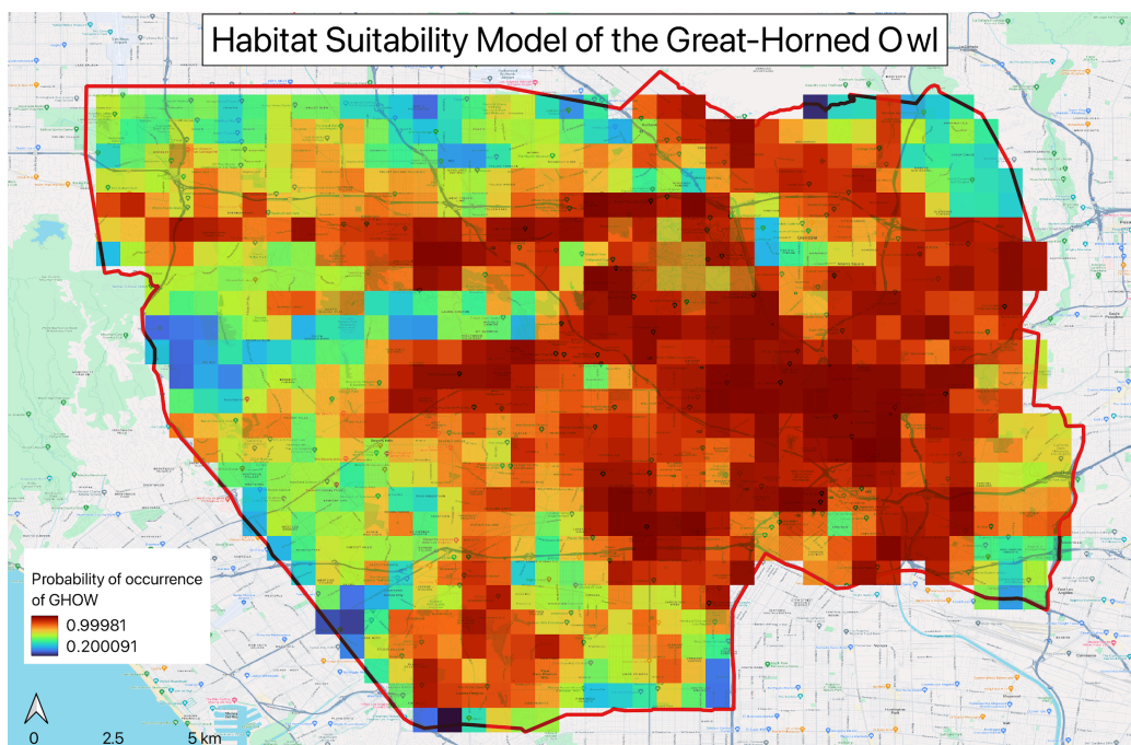
Figure 4. Habitat suitability model for the Great Horned Owl (GHOW) in the LA Raptor study area.
