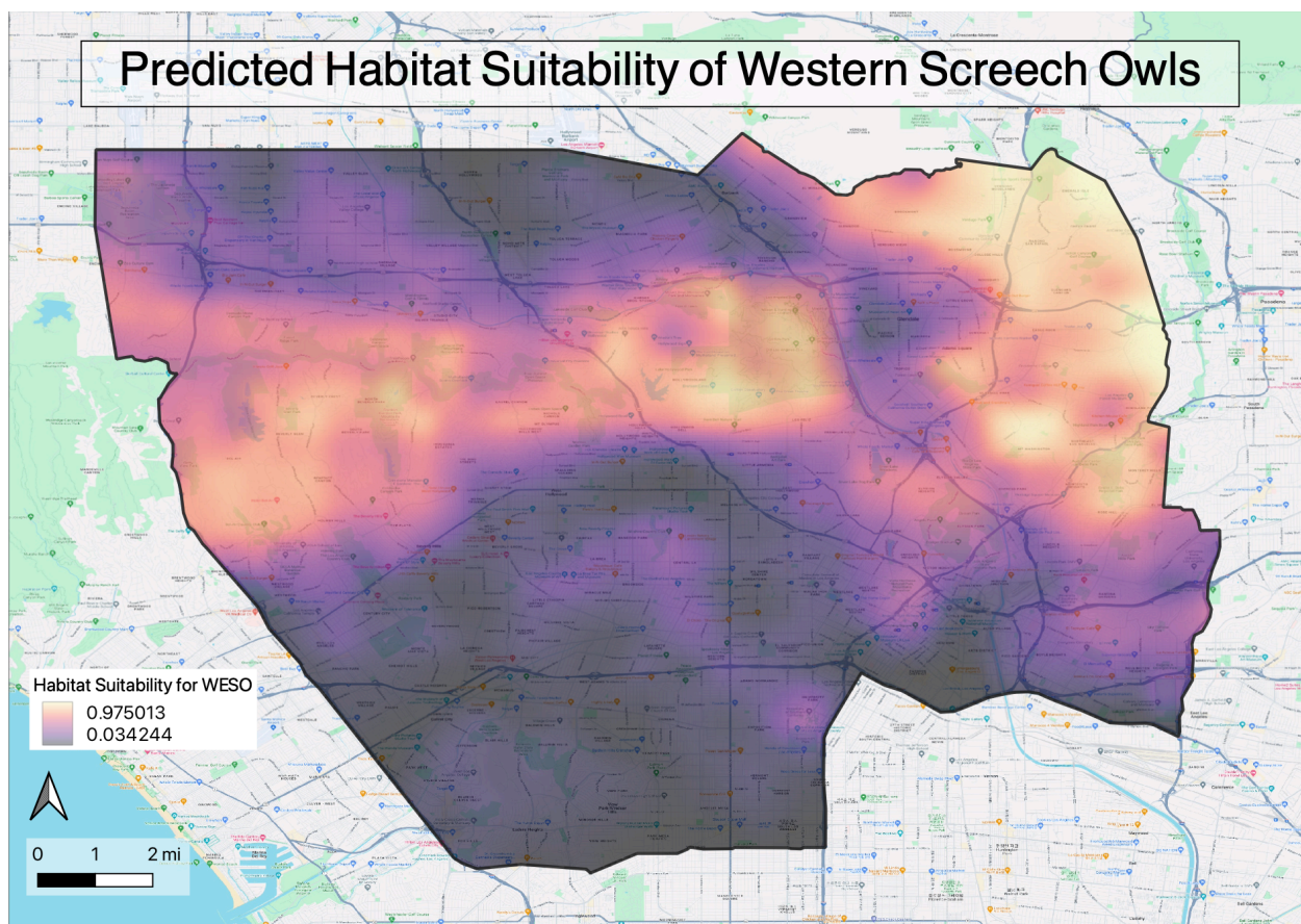
Figure 7. Habitat suitability model for the Western Screech-Owl (WESO) in the LA Raptor study area.
