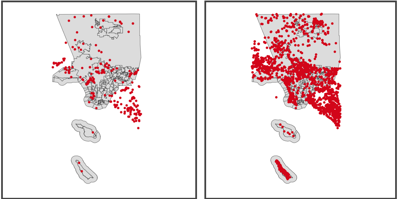
Figure 3. Presence data points downloaded from GBIF of the Barn Owl in Los Angeles County. The figure on the left (3a) shows the data points that were downloaded using the original GBIF code, while the figure on the right (3b) shows the data points from the final code that was used.
