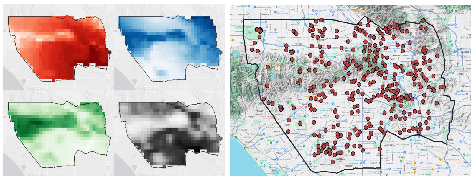
Figure 3. An example of the environmental layers used as inputs for MaxEnt habitat suitability modeling (left). From top right to top left clockwise: mean annual precipitation, impervious surface, canopy tree cover, and mean annual temperature (source: Dr. Ryan Harrigan). An example of presence-only data from iNaturalist and eBird is shown on the right of the figure. Each point indicates the presence of a Great Horned Owl.
