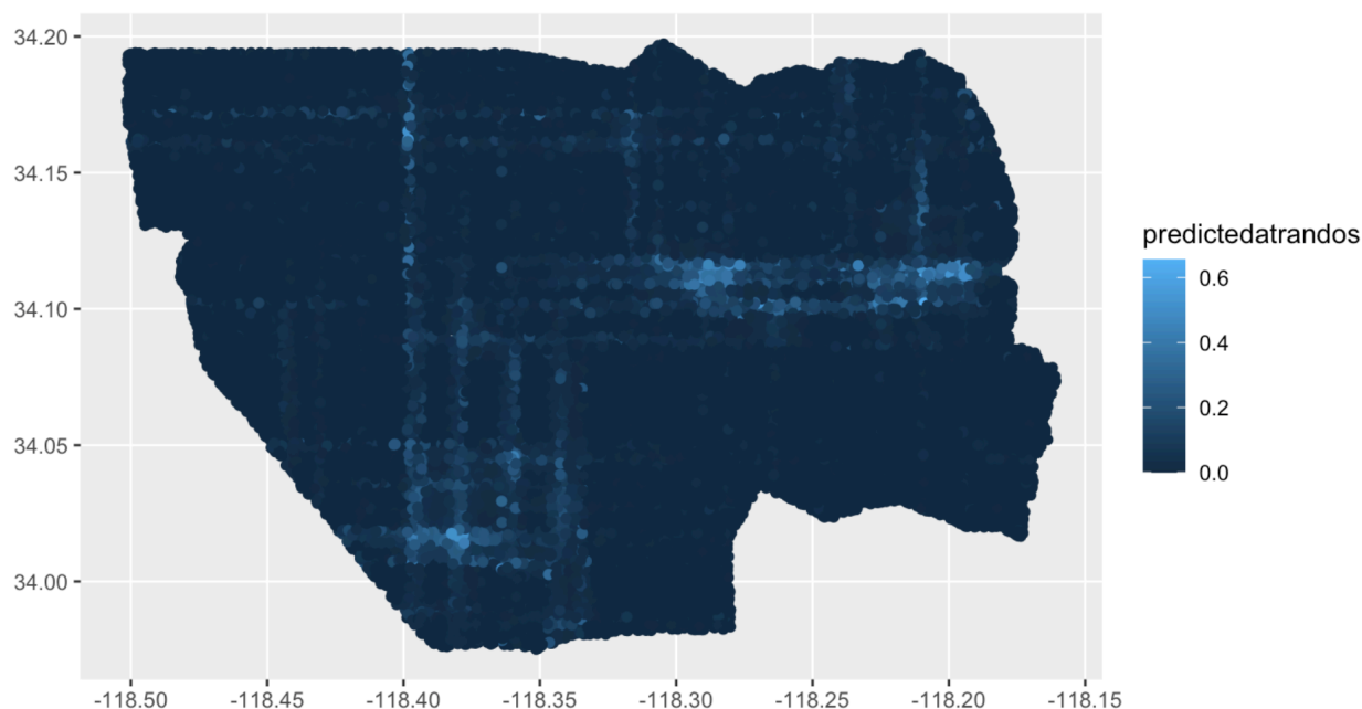
Figure 9. Random Forest model for the Barn Owl (BNOW) in the LA Raptor study area.
